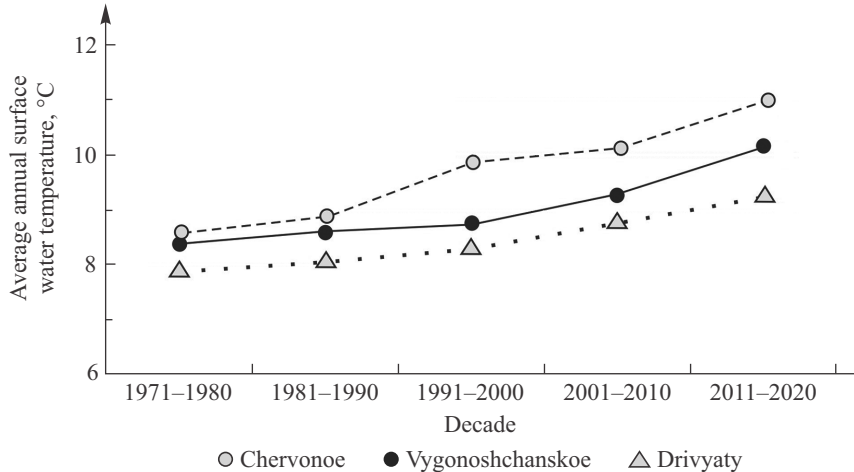
Fig. 7. Average annual surface water temperatures in selected lakes in Belarus in decade intervals in 1971–2020
