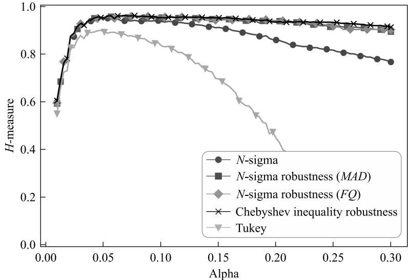
Fig. 4. Dependence H -measure on the contamination fraction with «shift» ( k = 4 ) contamination
