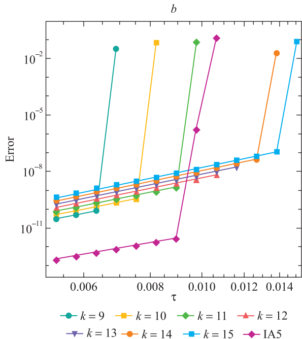
Fig. 3. Numerical experiment with HIRES problem. Six-step stabilised methods and implicit Adams method of order 6 (a). Stabilised methods of order 5 and implicit Adams method of the same order (b)
