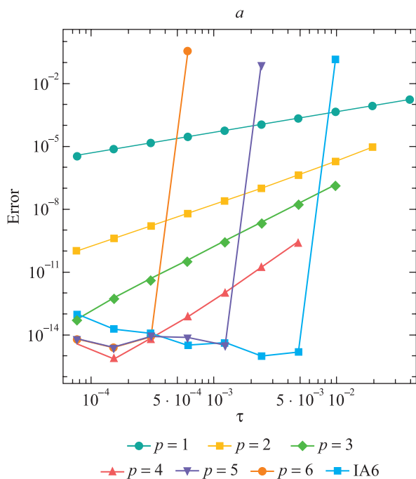
Fig. 3. Numerical experiment with HIRES problem. Six-step stabilised methods and implicit Adams method of order 6 (a). Stabilised methods of order 5 and implicit Adams method of the same order (b)
