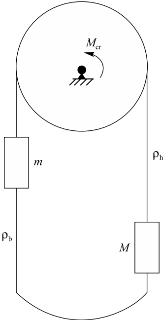
Fig. 3. Mine hoist scheme
