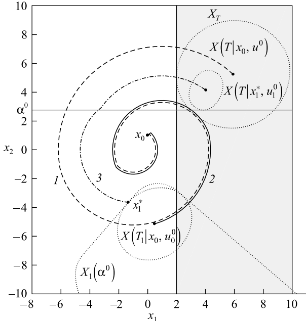
Fig. 1. Phase-plane solution representation of example 1.
