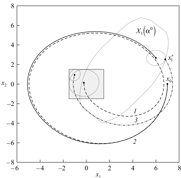
Fig. 3. Phase-plane solution representation of example 2. Trajectories under the optimal open-loop worst-case control (line 1), under the optimal initial open-loop control (line 2), and the optimal open-loop worst-case control on the interval after the closing instant for a sample state x_1^* (line 3)
