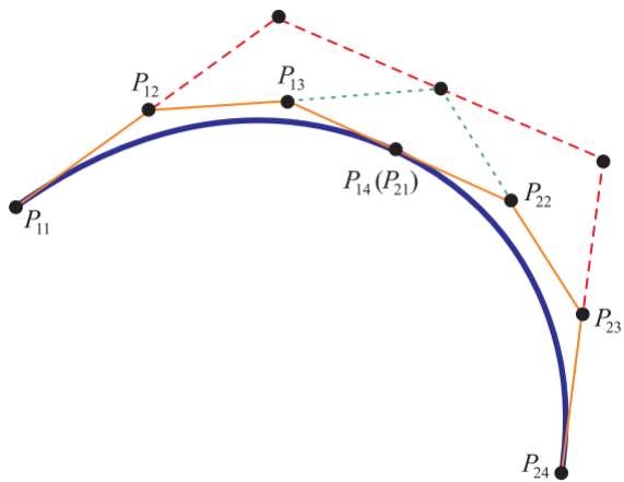
Fig. 6. Bezier curves B_1 and B_2
