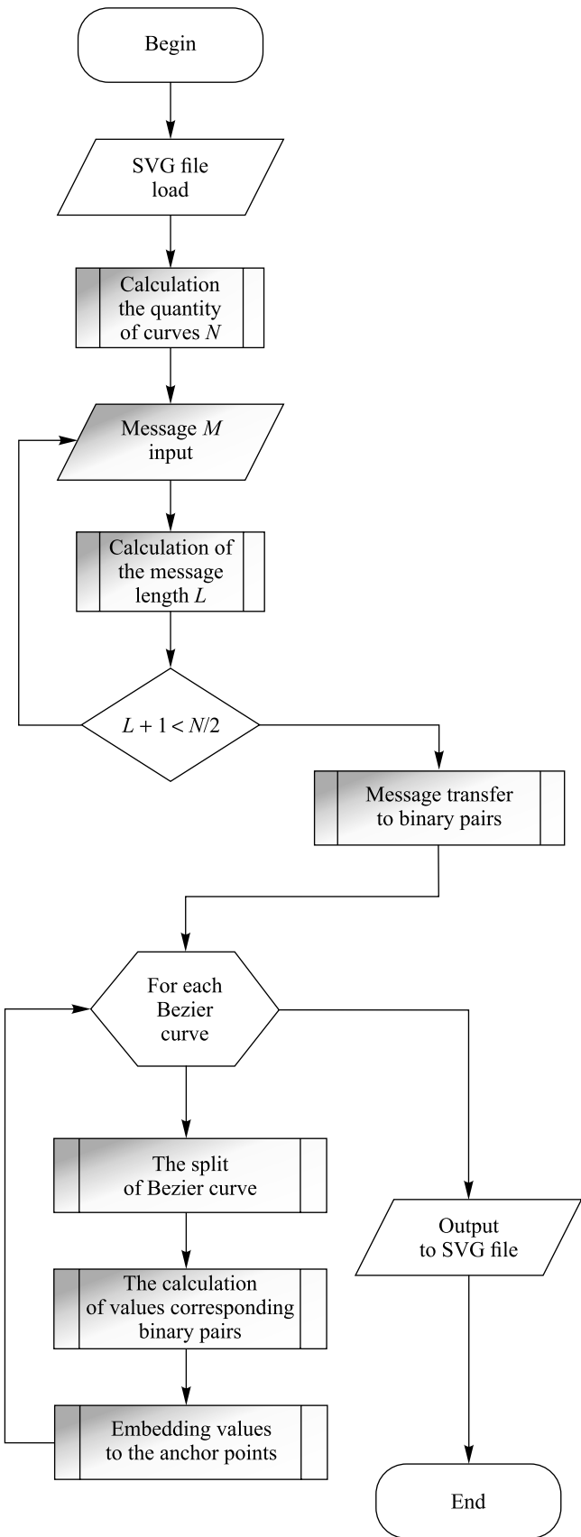
Fig. 7. Block diagram of the algorithm of hidden message embedding
