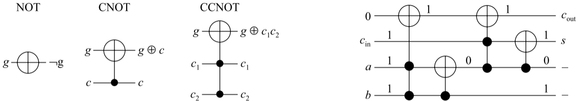
Fig. 1. Reversible gates of NCT library: a – reversible gates NOT, CNOT and CCNOT (Toffoli); b – realisation of 1-bit full adder by cascade of gates
