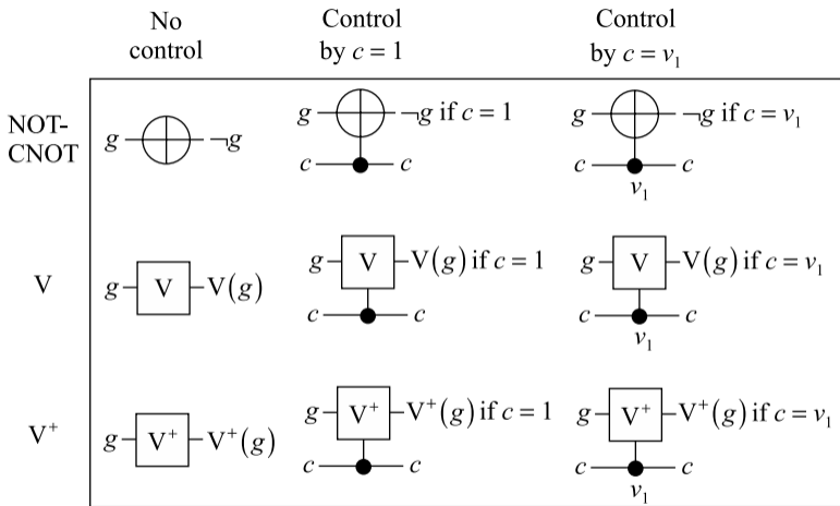
Fig. 2. Quantum gates of NCV and NCV- |v_1\rangle libraries:
