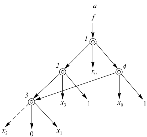
Fig. 8. Transforming optimised IFD to FIFD and then to reversible circuit: a – FIFD functionally equivalent to optimised IFD ( 1–4 denote the diagram node numbers); b – reversible circuit realising the FIFD (diagram node numbers are above columns)
