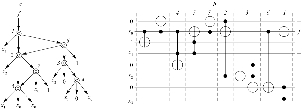
Fig. 9. Transforming immediate IFD to FIFD and then to reversible circuit: a – FIFD that is functionally equivalent to immediate IFD (1–7 denote the diagram node numbers); b – reversible circuit realising the FIFD (diagram node numbers are above columns)
