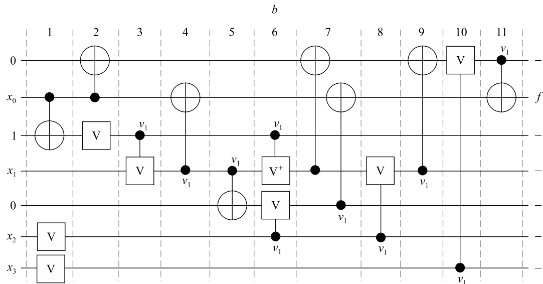
Fig. 10. Quantum circuits synthesised from optimised IFD (a) and ROBD (b). Numbers of columns indicate parallelisation steps
