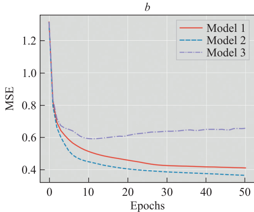
Fig. 1. The reconstruction loss (model 1 uses MSE and MSPE, model 2 uses MSE only, model 3 uses only MSPE as the loss): a – train part; b – test part
