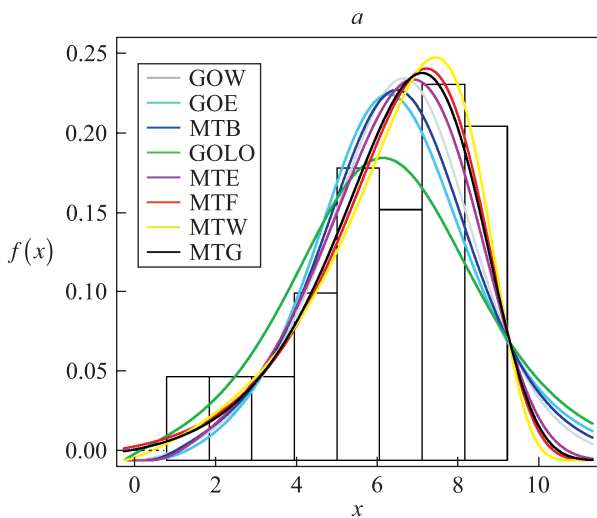
Fig. 5. Empirical estimate for the second dataset: a – empirical densities; b – empirical CDFs
