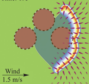
Fig. 4. Fire spread in the case of three fuelbreaks with 18 \text{ m}^2 each at the following time points: 65 ( a ), 130 ( b ), 195 ( c )
