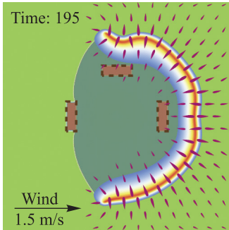
Fig. 6. Fire dynamics for the rectangular fuelbreak geometry at the following time points: 65 ( a ), 130 ( b ), 195 ( c )
