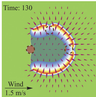
Fig. 10. Fire dynamics for the circular fuelbreaks at 1.5 m/s wind velocity at the following points: 65 ( a ), 130 ( b ), 195 ( c )
