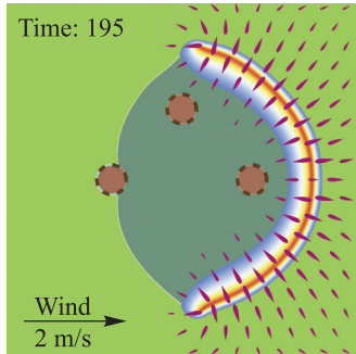
Fig. 11. Fire dynamics for the circular fuelbreaks at 2 m/s wind velocity at the following points: 65 ( a ), 130 ( b ), 195 ( c )
