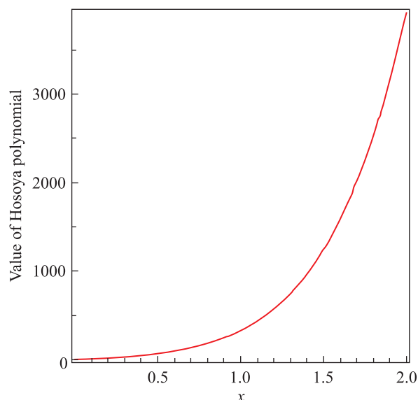
Fig. 2. The plot of the Hosoya polynomial of the CHDN3[5] for 0 \leq x \leq 2
