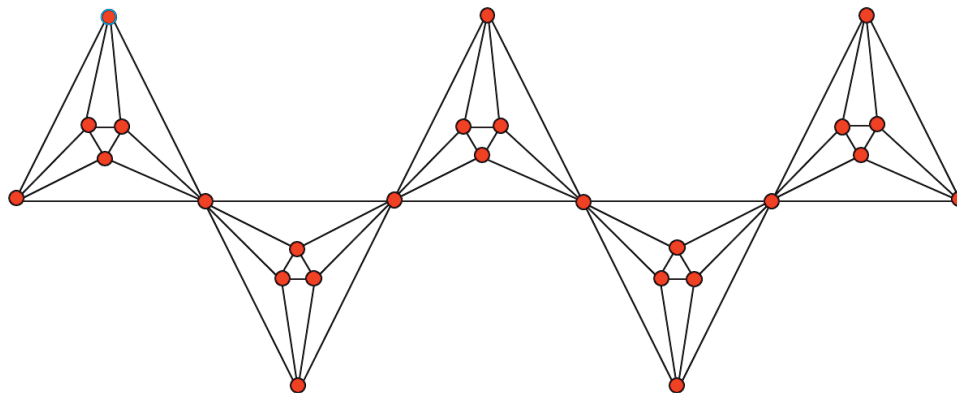
Fig. 1. The third type of chain hex-derived network of dimension 5 ( CHDN3[5] )
