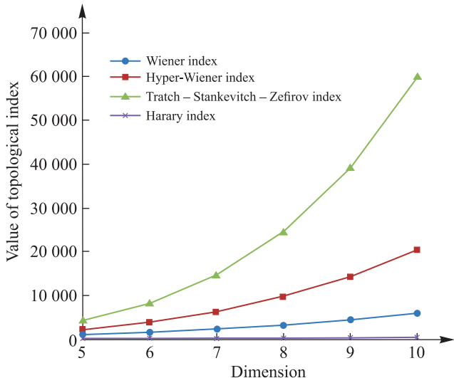
Fig. 3. The plot of the Wiener, hyper-Wiener, Tratch – Stankevitch – Zefirov, and Harary indices of the CHDN3[n] network for different values of n ( 5 \leq n \leq 10 )
