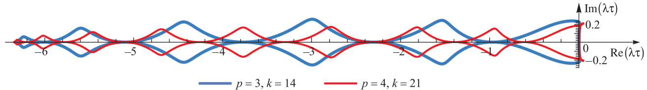
Fig. 1. Root locus curves (3) of the methods with an extended stability interval
