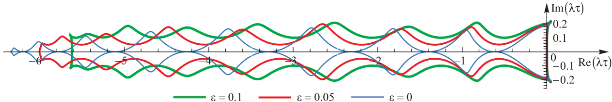
Fig. 3. Root locus curves (3) of the damped methods with p = 4 , k = 21
