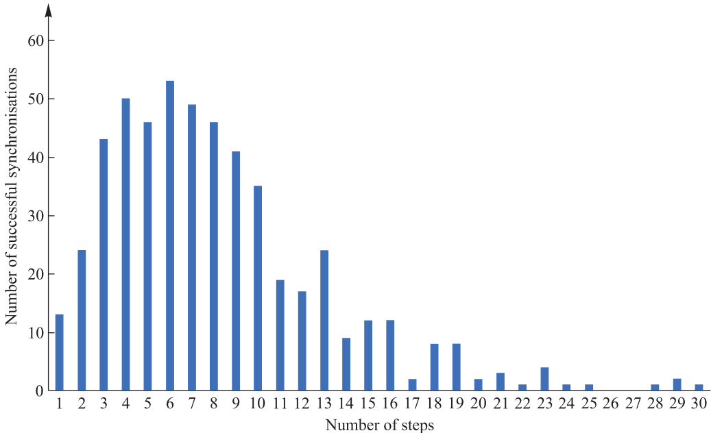
Fig. 3. Main part of the distribution of the number of TPOM ( N = 6 , K = 6 , L = \pm 6 ) in accordance with the number of steps ( t' ) until the moment comes when \mathbf{W}^A = \mathbf{W}^B for 1168 simulations
