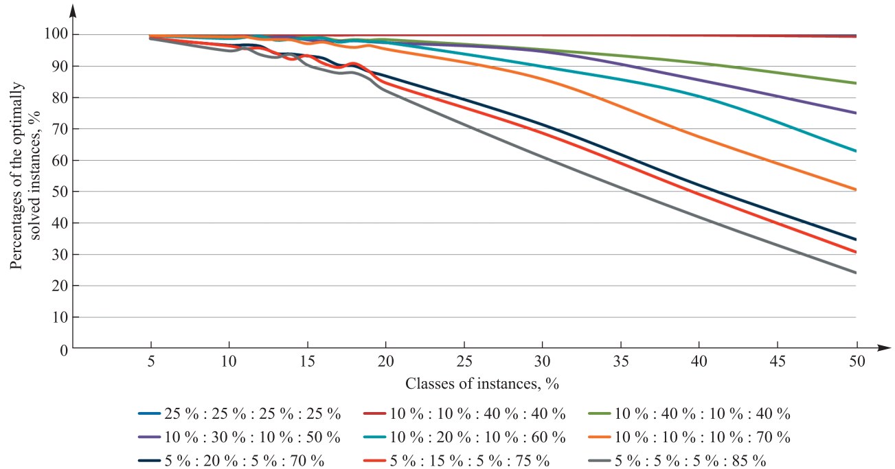
Percentages of the optimally solved instances for different classes of instances
