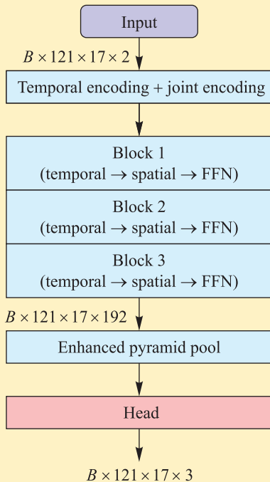
Fig. 3. 3D pose estimation framework using the MTSA-former model
