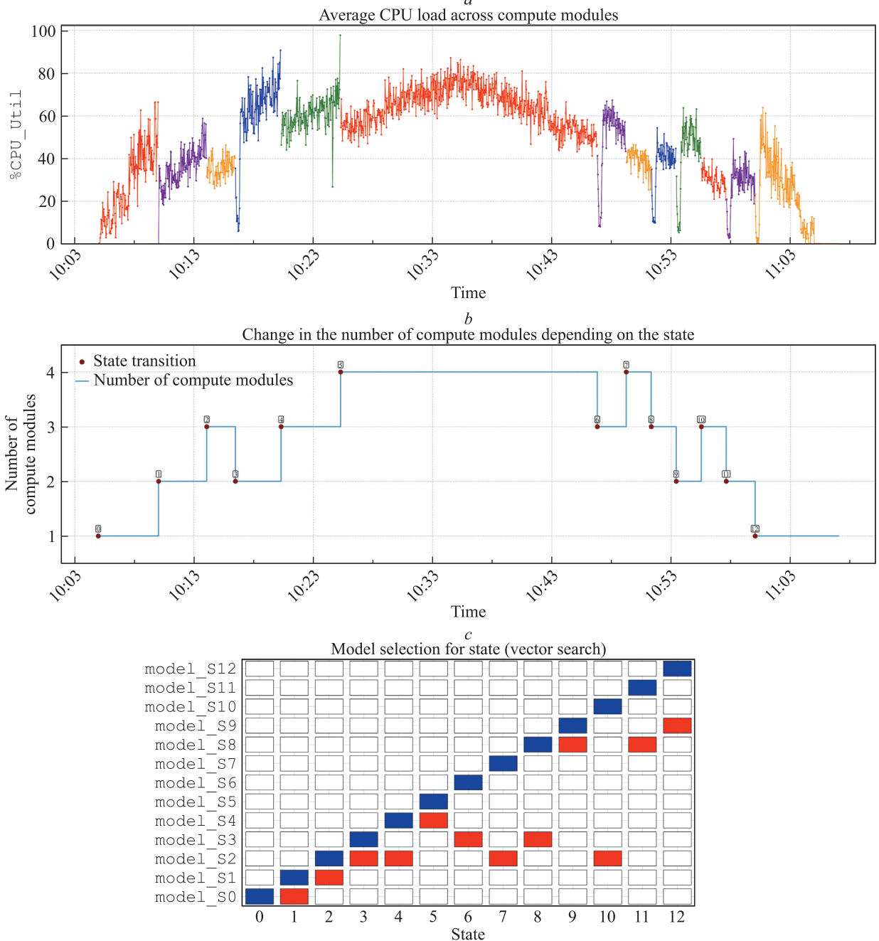
Fig. 11. Illustration of the operation of algorithm A90.50.R60P70L60_70FNNL_VEC1 ( a , b ) and model selection using vector search ( c ) for profile PROFILE2_DISP20
