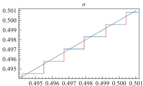
Fig. 3. Comparison between empirical CDF F_N of the p -values generated by Frequency test for n = 2^{20} and uniform CDF ( a ). Deviation of the empirical CDF F_N of the p -value distribution of the Frequency test from continuous uniform CDF ( b )
