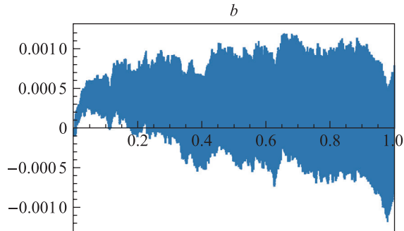
Fig. 3. Comparison between empirical CDF F_N of the p -values generated by Frequency test for n = 2^{20} and uniform CDF ( a ). Deviation of the empirical CDF F_N of the p -value distribution of the Frequency test from continuous uniform CDF ( b )
