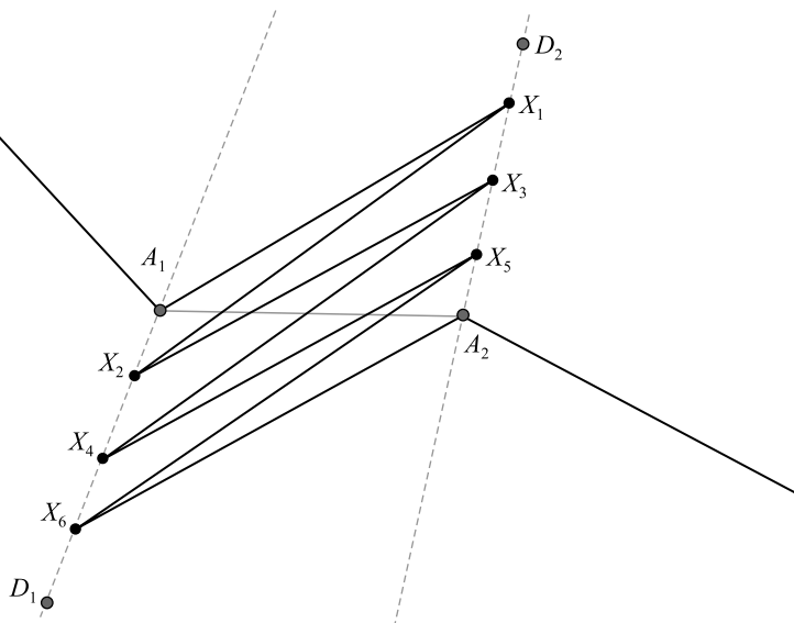
Рис. 2. Преобразование звена [A_1A_2] Fig. 2. Transformation of segment [A_1A_2]
