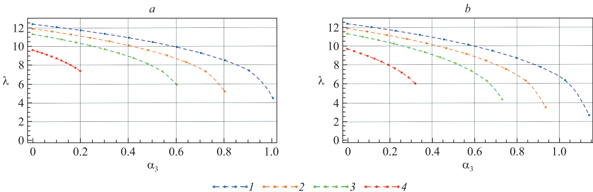
Fig. 5. The first positive eigenvalue \lambda versus the vdW parameter \alpha_3 for different values of the voltage parameter \beta calculated in the framework of the LDL (a) and QDL (b) models: \beta = 0 (1), \beta = 0.15 (2), \beta = 0.3 (3), \beta = 1.0 (4)
