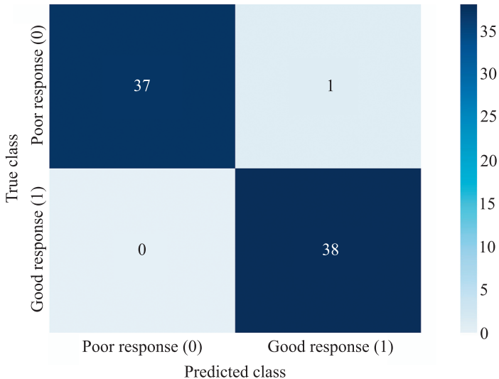
Fig. 2. Confusion matrix
