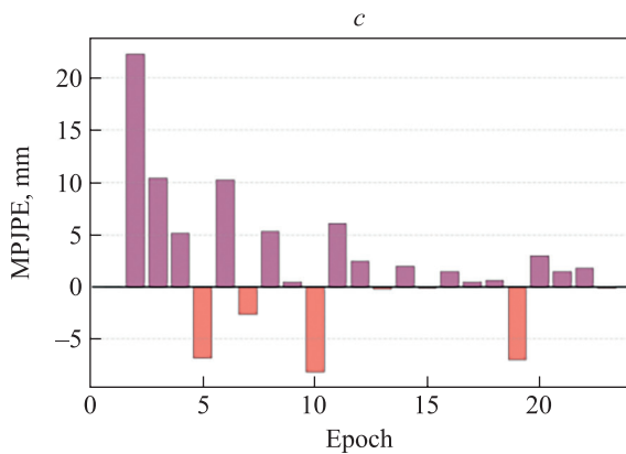
Fig. 5. Variations and convergence trends of key loss metrics during the training of the MTSA-former model: a – training and validation MPJPE; b – total loss; c – epoch-to-epoch validation change; d – best validation MPJPE progress
