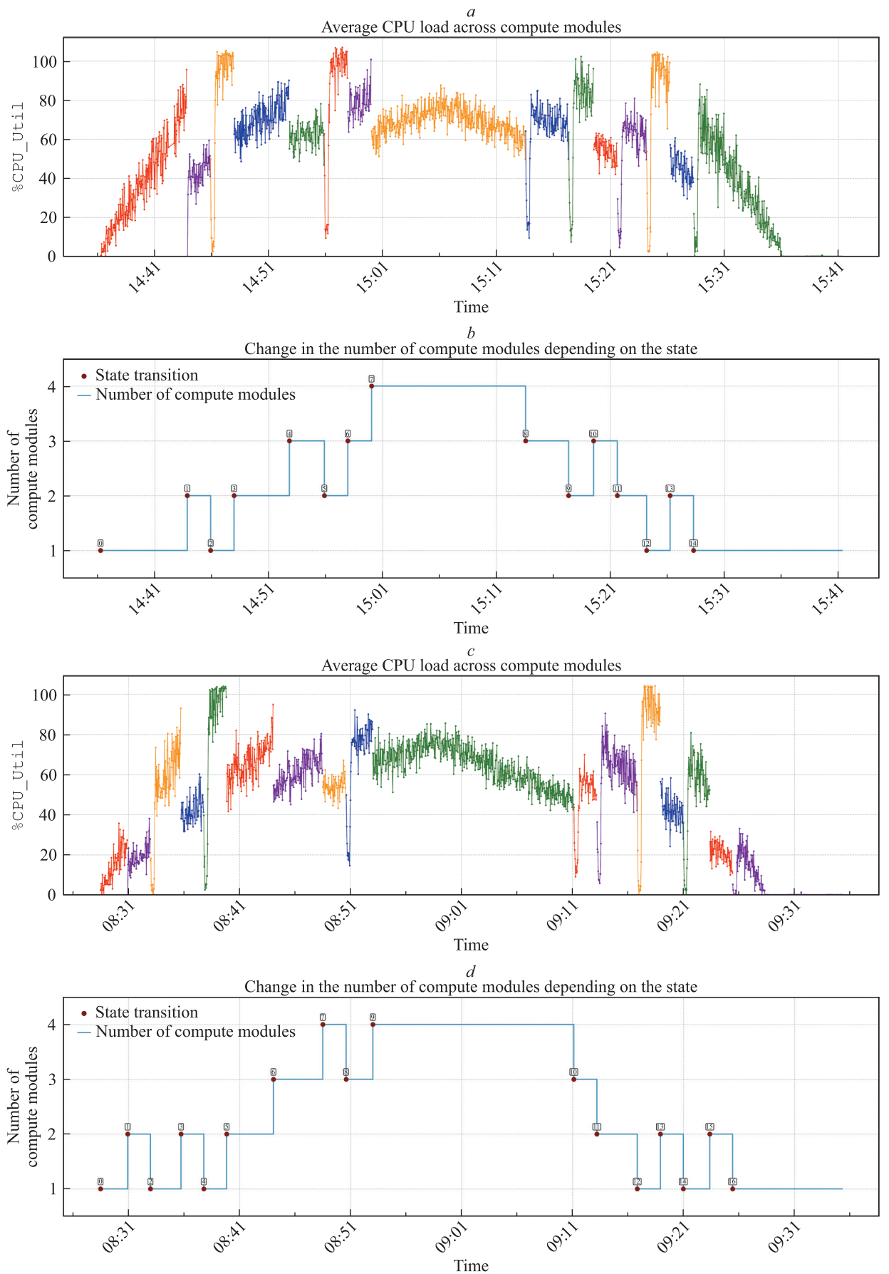
Fig. 8. Illustration of the operation of algorithms A90.50.R60 ( a , b ) and A90.50.R60P70F ( c , d ) for profile PROFILE2
