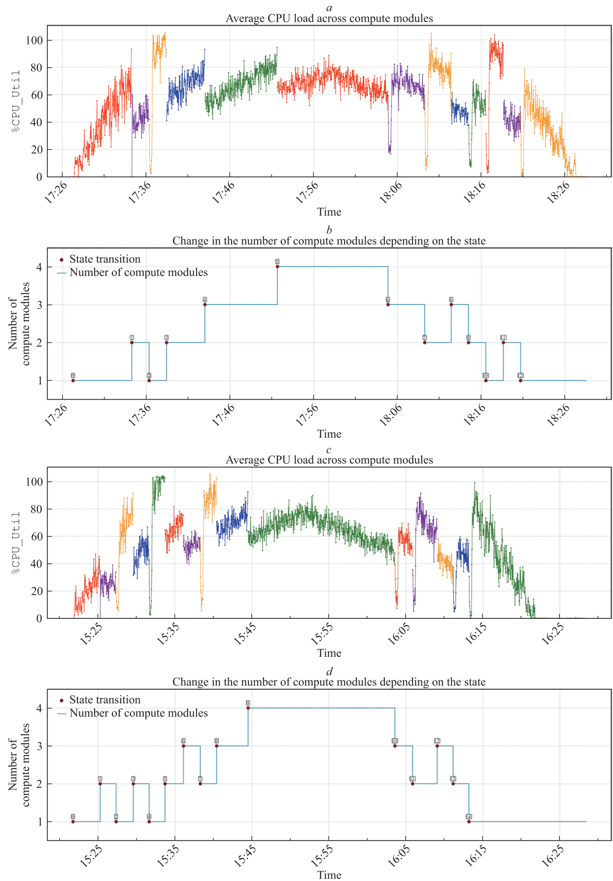
Fig. 10. Illustration of the operation of algorithms A90.50.R60 ( a , b ) and A90.50.R60P70F ( c , d ) for profile PROFILE2_DISP20
