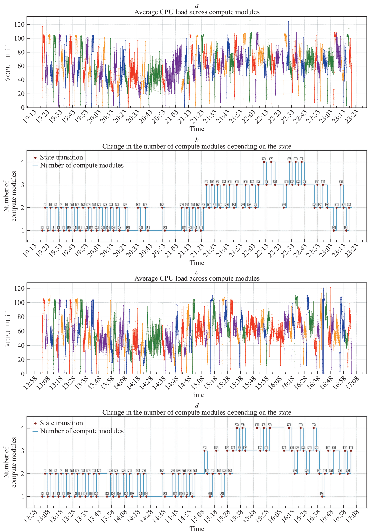
Fig. 12. Illustration of the operation of algorithms A90.50.R60 (a, b) and A90.50.R60P70F (c, d) for profile APROFILE1
