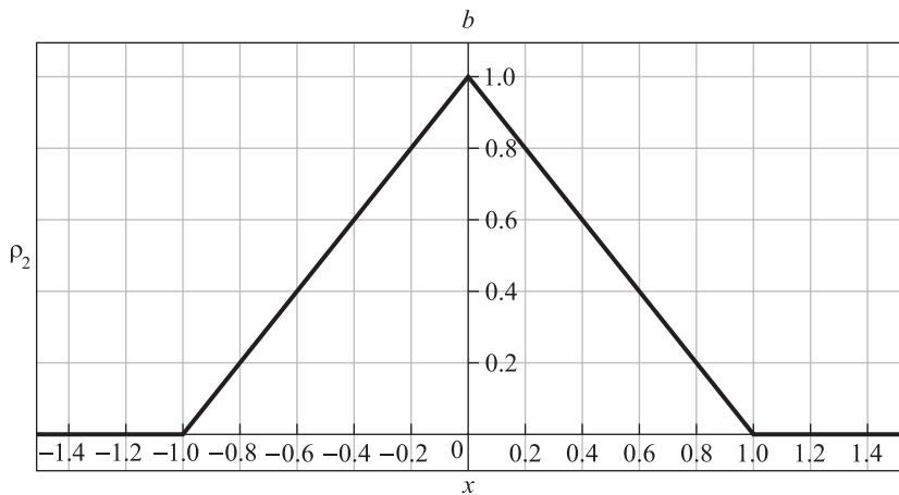
Fig. 4. Functions \rho_1(x) (a) and \rho_2(x) (b)
