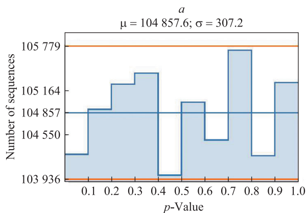
Fig. 2. Comparison between expected deviation and measured deviation in the distribution of p -values in the interval [0,1] for the Frequency test ( a ) and the Binary matrix rank test ( b )
