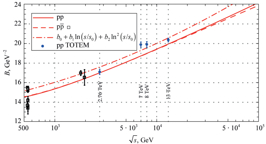
Fig. 2. pp and p\bar{p} elastic slope B(s) calculated from the fitted model (1)–(4)
