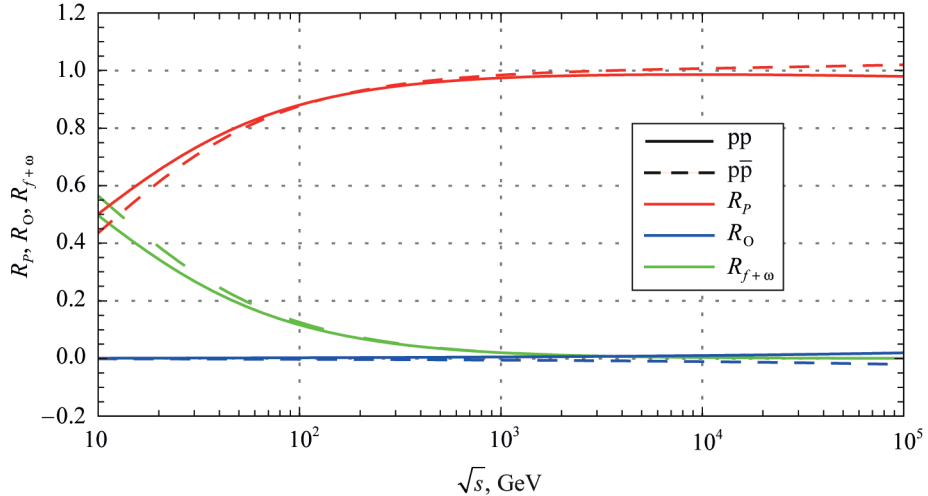
Fig. 4. Relative contribution from different components of the amplitude to pp and \bar{p}p cross sections calculated from the model (1)–(3), (7)
