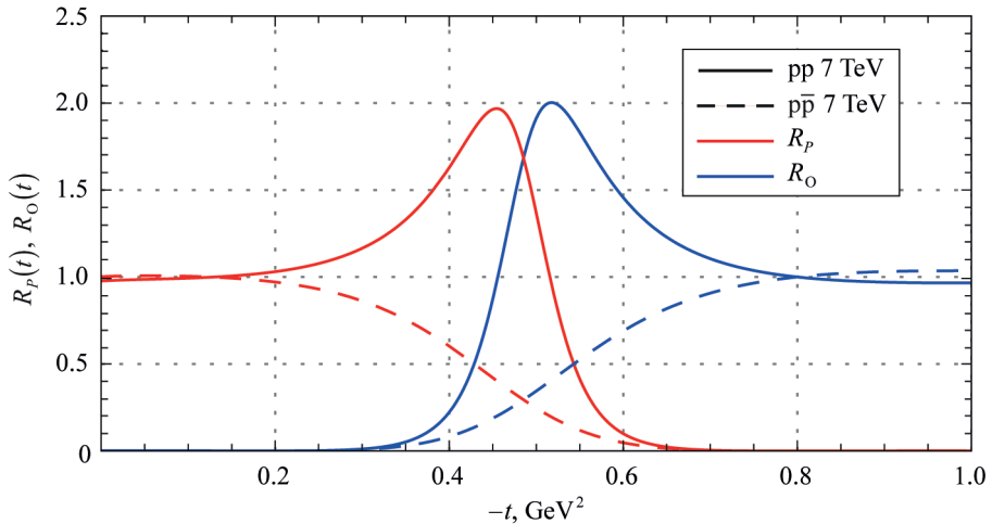
Fig. 5. Relative contribution from the pomeron and from the odderon to the pp and p\bar{p} differential cross sections at 7 TeV calculated from the model (1)–(3), (8)
