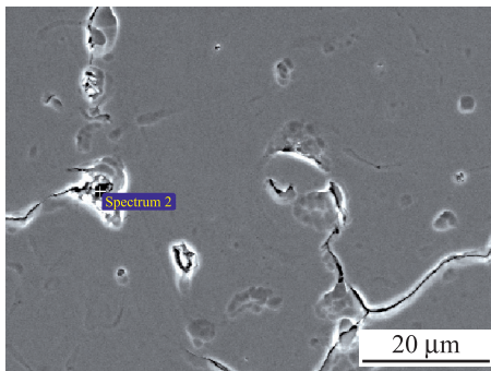
Fig. 2. SEM images of the surface of FeCrAl doped with yttrium + molybdenum after sputtering ( a ), detail of the surface with cracks along grain boundaries ( b ) and precipitates ( c ) and the EDS analyses from the points marked in the images ( b , c )
