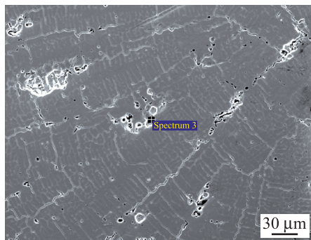
Fig. 3. SEM images of the initial surface of FeCrAl doped with molybdenum + yttrium + zirconium ( a , b ), detail of the surface after sputtering ( c ) and the EDS analyses from the points marked in the images ( b , c )
