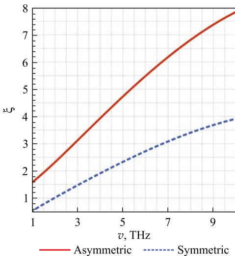
Fig. 3. The value of the propagation coefficient \xi in the plane of graphene layers with the dielectric spacer thickness 10 nm for \Gamma_{\text{trans}} = 13 THz
