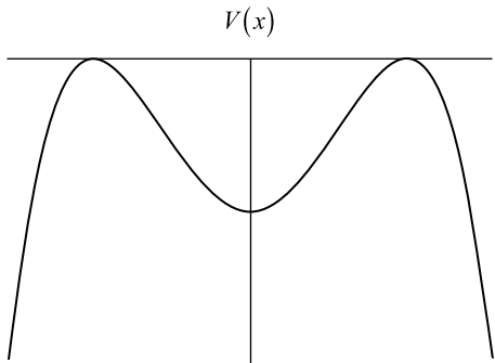
Fig. 2. Inverted by Wick rotation potential
