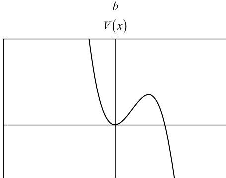
Fig. 4. Potential of a system with metastable state: a – Lorentzian version; b – Euclidean version
