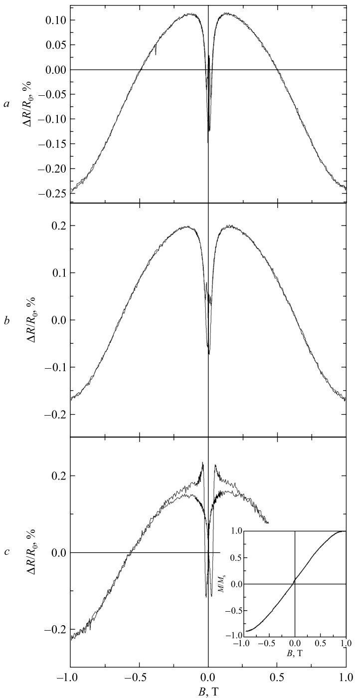
Fig. 2. Magnetoresistance hysteresis loops of the Corbino permalloy disk at \phi = 90^\circ , measured at different temperatures: a – 100 K; b – 50 K; c – 2 K (the inset in figure c shows the magnetisation hysteresis loop at T = 2 K)
