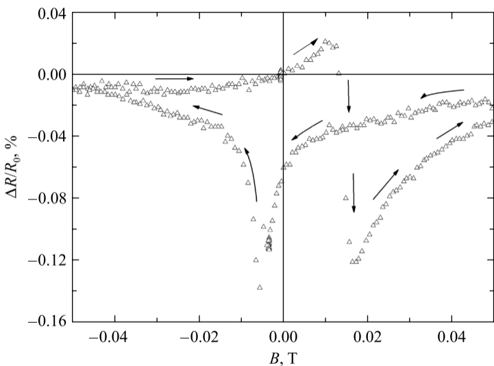
Fig. 3. Magnetoresistance hysteresis loop for the Corbino permalloy disk in a weak magnetic field at \varphi = 0^\circ and T = 2 K
