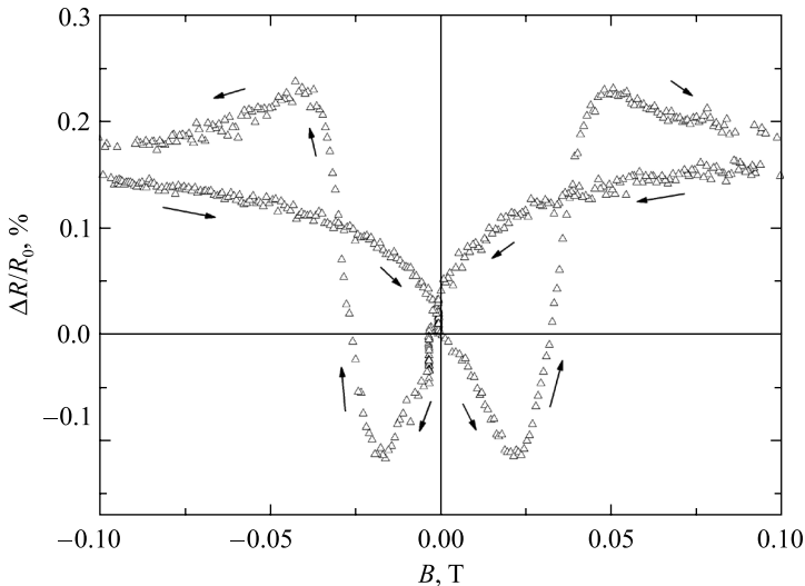
Fig. 4. Magnetoresistance hysteresis loop for the Corbino permalloy disk in a weak magnetic field at \varphi = 90^\circ and T = 2 K
