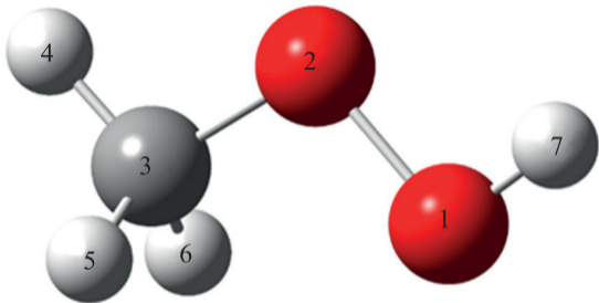
Fig. 1. Configuration of the MHP molecule, in which the values of the torsional coordinates \alpha of the hydroxyl group and \theta methyl group are considered to be zero
