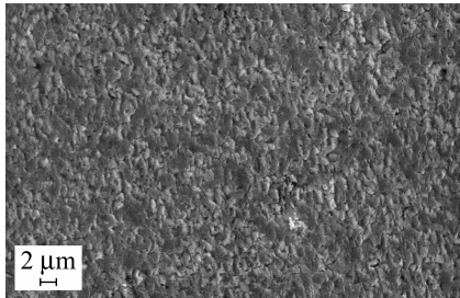
Fig. 2. Scanning electronic images of the surface of InSb films formed by explosive thermal evaporation at deposition temperatures: a – 375 °C; b – 460 °C
